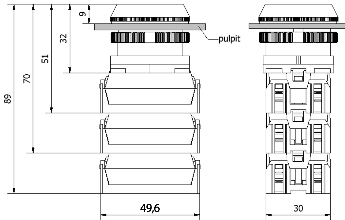
NEF30-K
