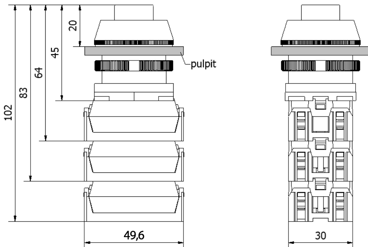
NEF30-UW
