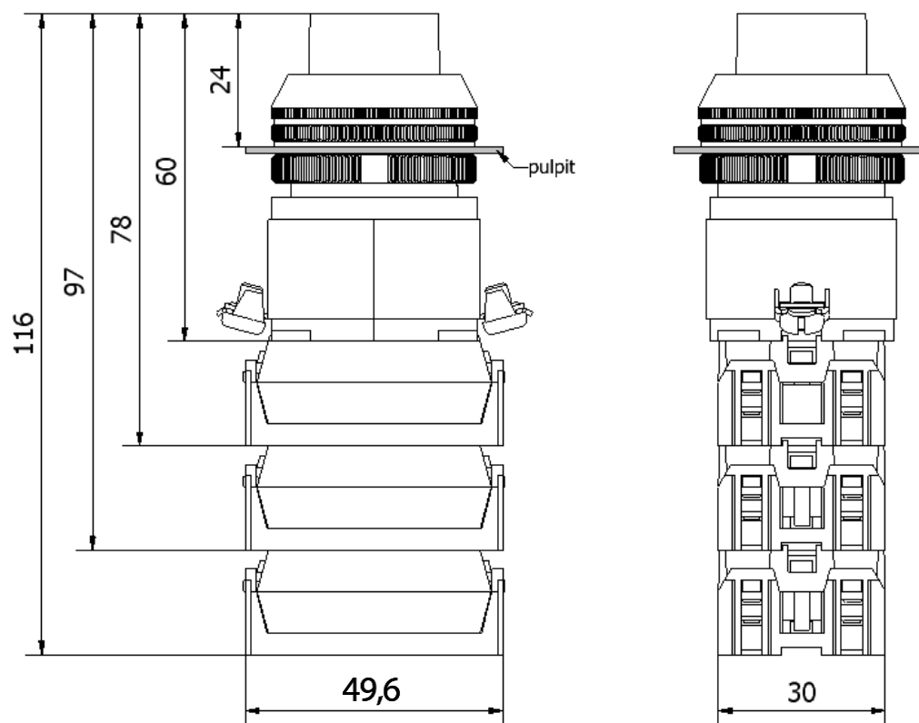
NEF30-WL, NEF30-WLD, NEF30-UWL, NEF30-UWLD
